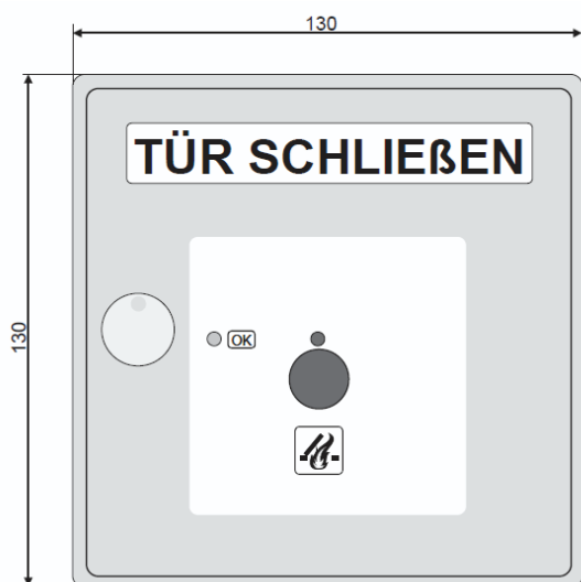
Maßbild Dimensioned drawing
