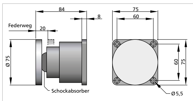
Teleskopanker ATV 75
