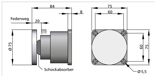
Teleskopanker ATV 75
