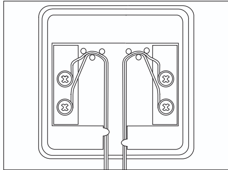
Abb. 1: Verbinden externer Taster
